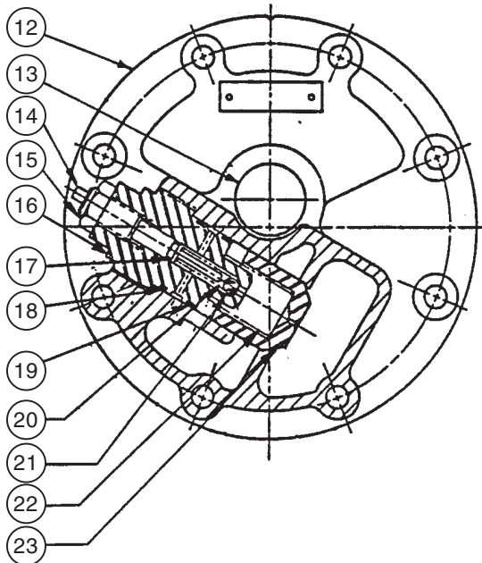
Section through relief valve.
