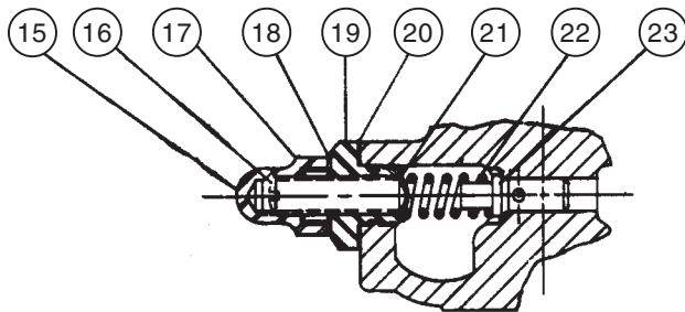
Section through relief valve.
